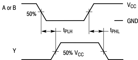
Figure 3. Switching Waveforms
