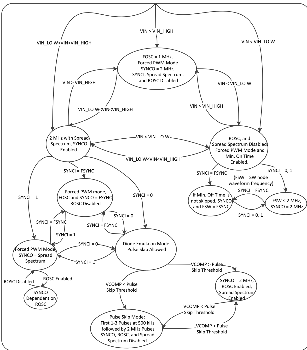
Figure 22. NCV891930 State Diagram – Dependent Switching Logic
