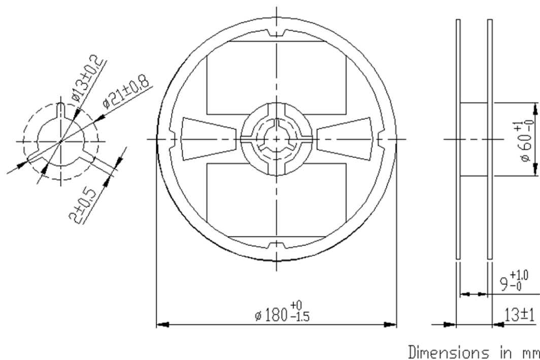
Carrier Tape
